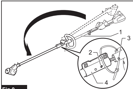
Fig.9 ► 1. Upper pipe 2. Stopper hole 3. Stopper pin 4. Joint
